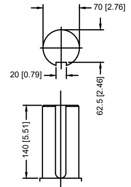
DRIVE SHAFT
