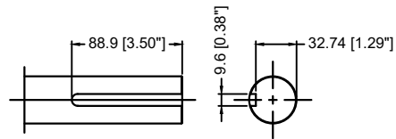
SHAFT DETAIL
