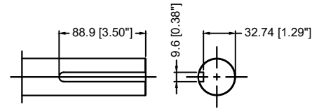
SHAFT DETAIL
